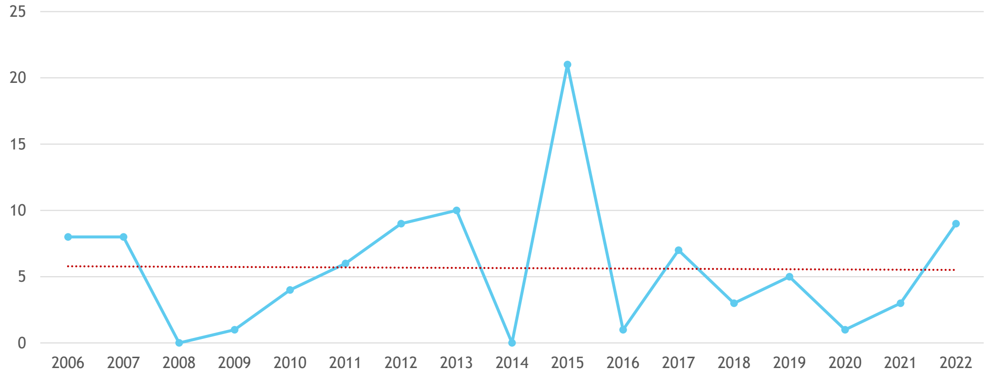
Number of tropical days in Modra (from july to september)
