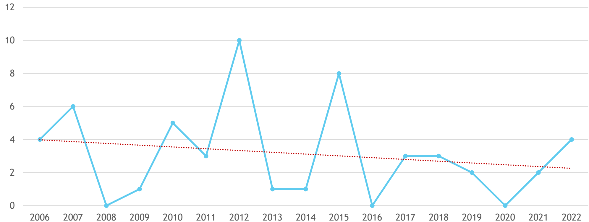
Number of tropical nights in Modra (from july to september)
